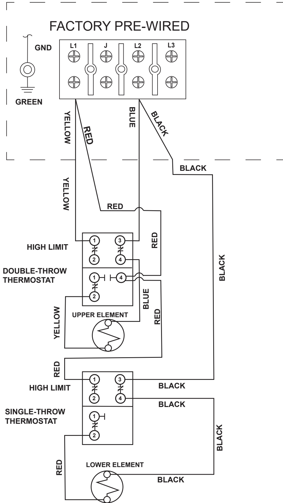
Figure 8. Wiring Diagram
