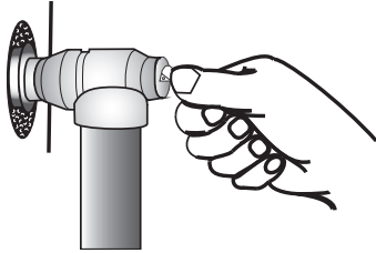
Figure 5. Testing the Temperature-Pressure Relief Valve
