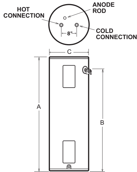
Figure 2. Rough-in Dimensions
