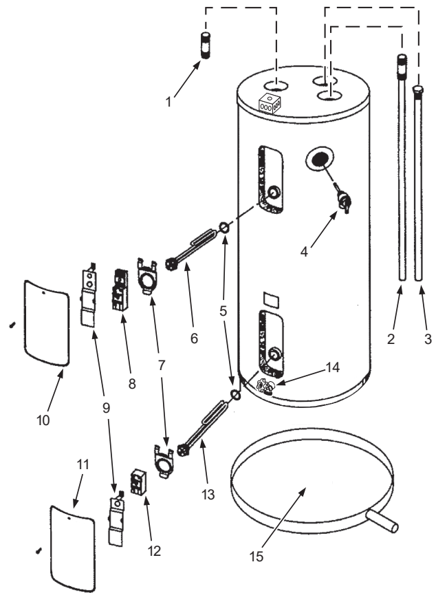
Figure 6. Repair Parts
