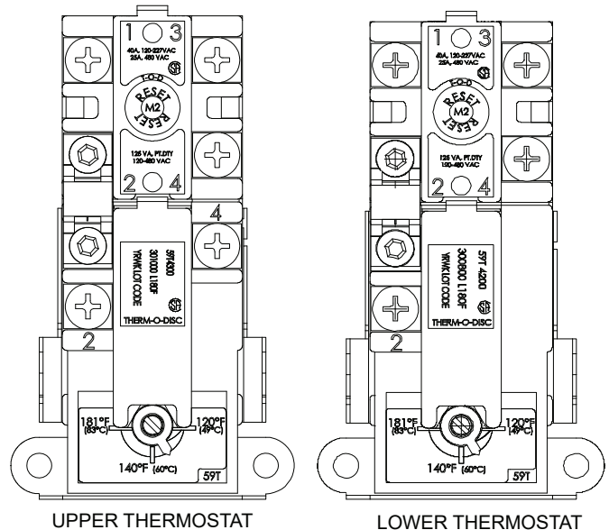
Figure 3. Thermostat Controls
