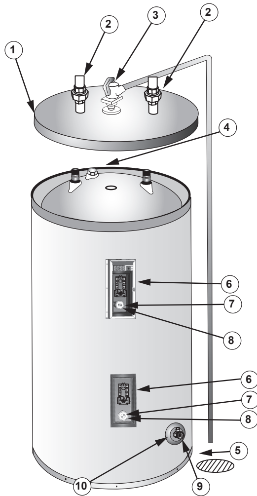
Figure 7. Leakage Checkpoints
