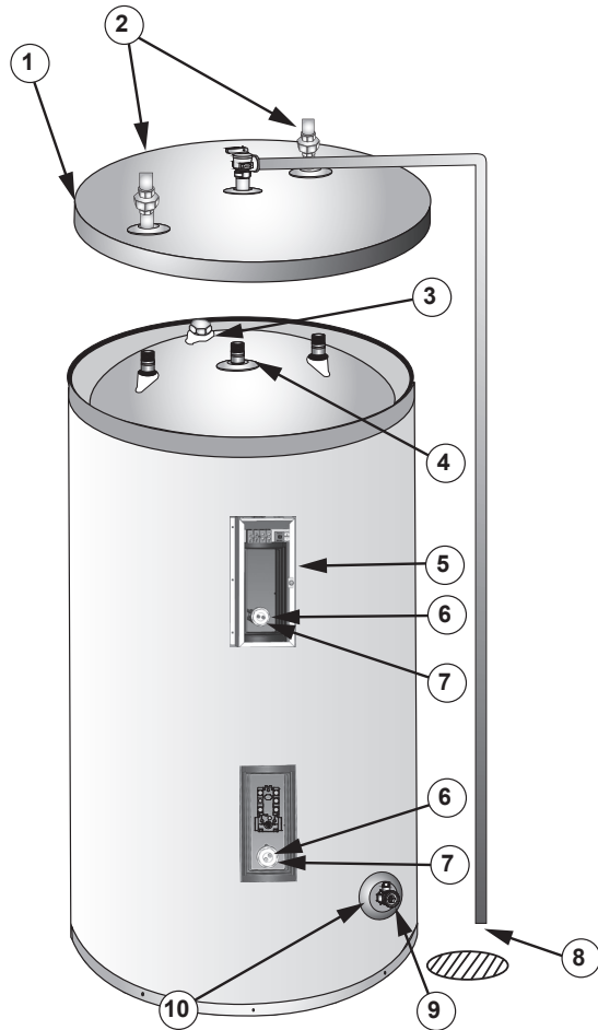
Figure 7. Leakage Checkpoints
