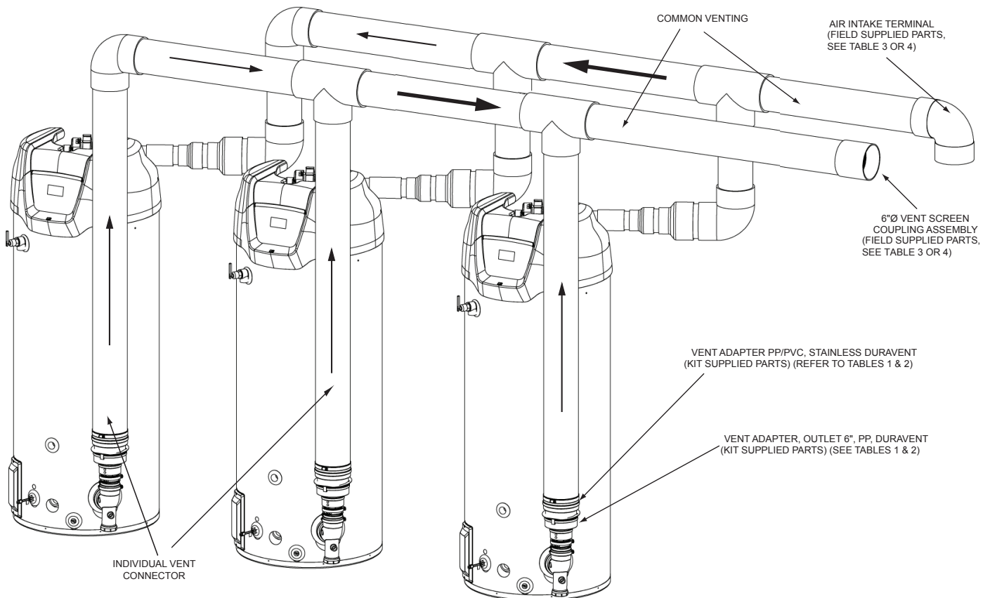
FIGURE 4. DEFINITION OF SYSTEM SECTIONS - PVC
