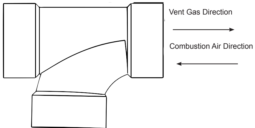
FIGURE 5. SANITARY TEE
