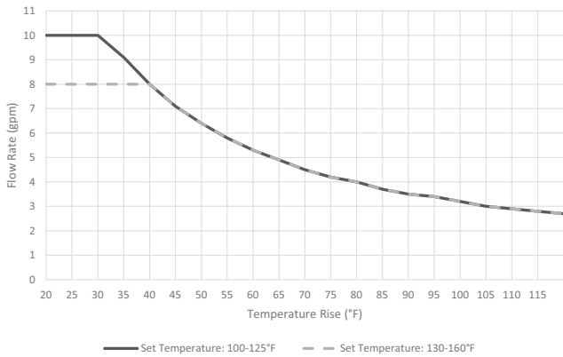
510C: Flow Rate vs. Temperature Rise
